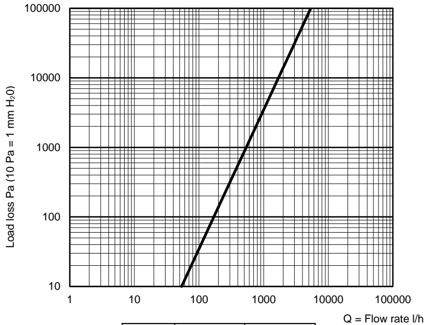
Load losses diagram
